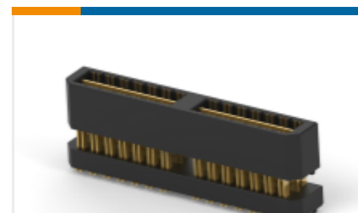
TE Part # 1-1658438-2 MSB0.80PL14ASY56DP,-,10,VCTY
